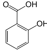
2. Salicylic acid
