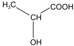
1. Lactic acid
