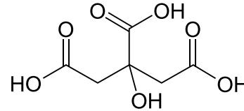
3. Citric acid
