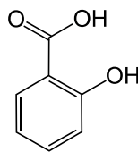
2. Salicylic acid
