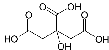
3. Citric acid
