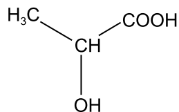
1. Lactic acid
